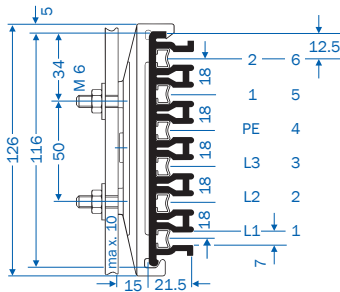
Installation: lateral
